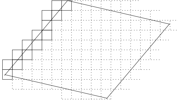
Figure 1: The border effect on V^{-1}(\sigma)
