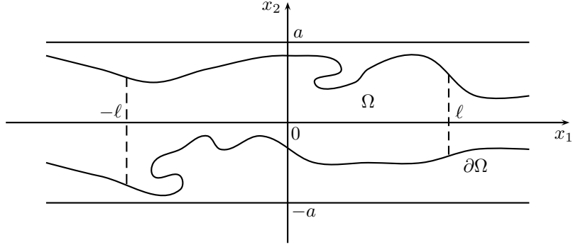
FIGURE 1. \Omega
