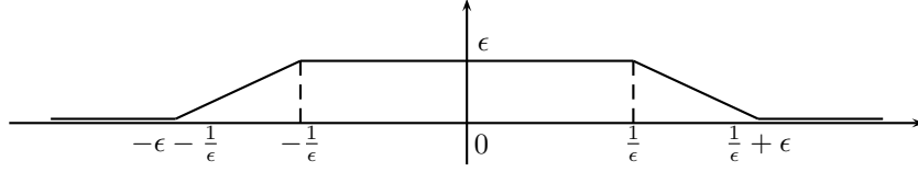
FIGURE 2. \rho_\epsilon
