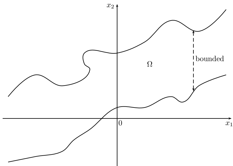
FIGURE 3. General domain
